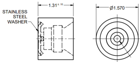
FEMALE BASE
