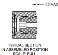
MALE STEM
