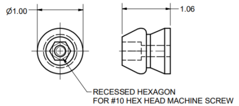
MALE STEM
