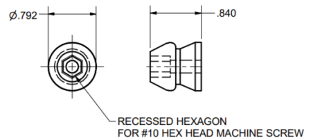
MALE STEM
