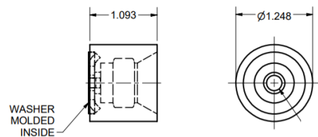
FEMALE BASE
